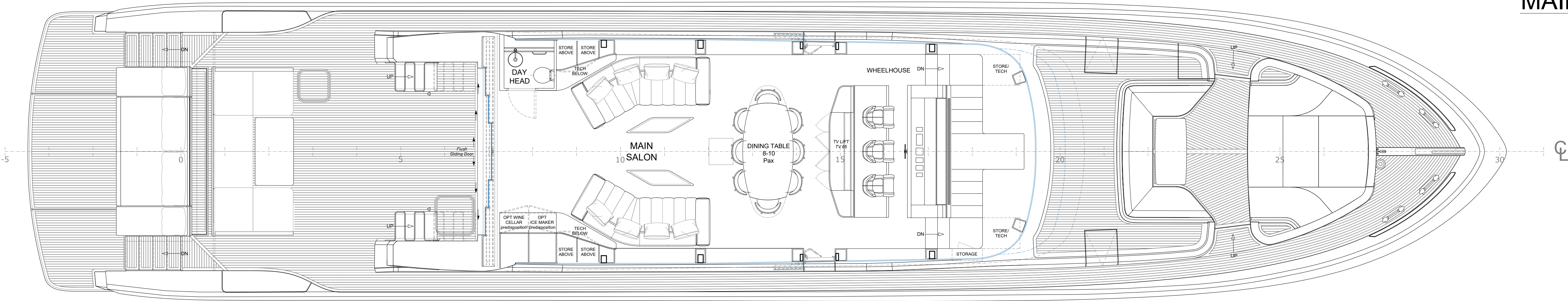
MAIN DECK
